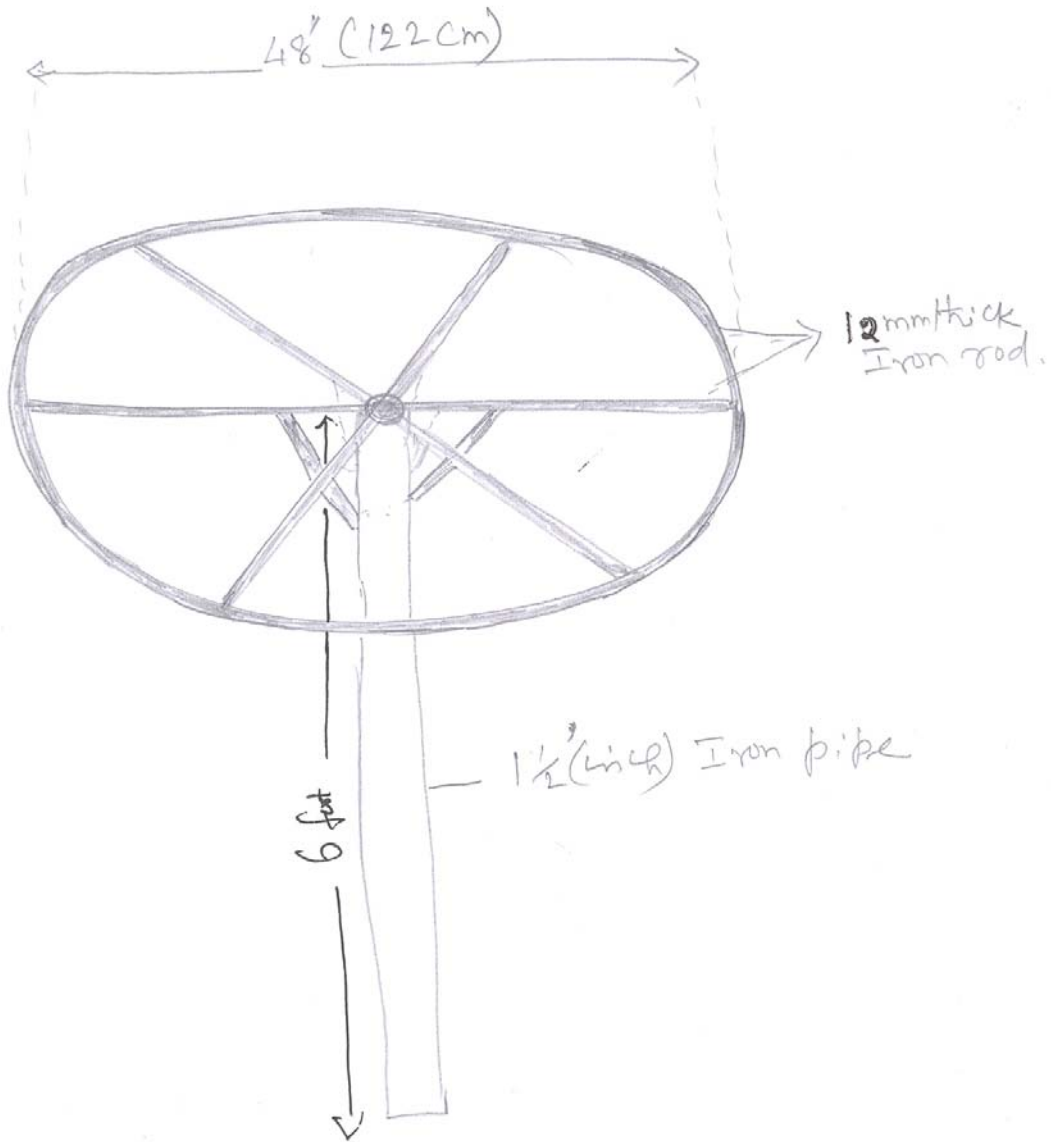
"Iron field board Supporting Structure" (Specification)
